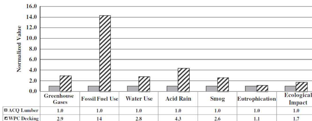
Figure 4: Cradle to grave comparison of a number of indicators for the average sized wooden deck (for an American family). Source: (Bolin, C.A and Smith, S. 2011)
