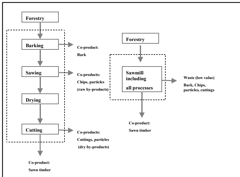
Figure 3. Different allocation of energy consumption to different products from sawmill (source: Jungmeier et al.)
