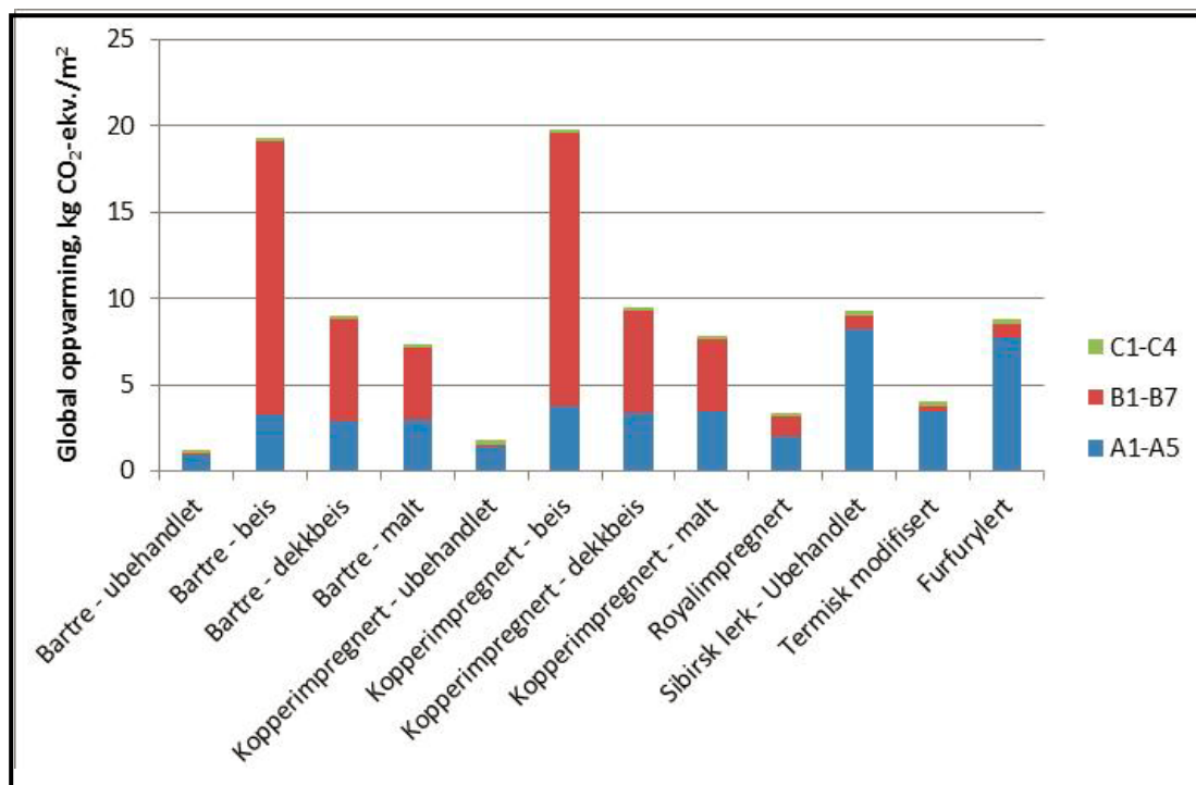
Figure 4. Emissions of greenhouse gases for each type of cladding. Total for the production, installation and use phases. The figures are from the report "Miljøanalyse av trefasader" (Environmental analysis of wood facades – SINTEF Byggforsk, the Norwegian Institute of Wood Technology and the Norwegian Forest and Landscape Institute) 27 . Phases A1-A5 include raw material extraction, production and installation of the cladding including transport. Phases B1-B7 include the use phase (emissions from the surface treatment and maintenance). Phases C1-C4 include demolition and waste management. According to the report, the results for Royal impregnated wood are too low, since energy use during impregnation with oil is not taken into account due to lack of data.
